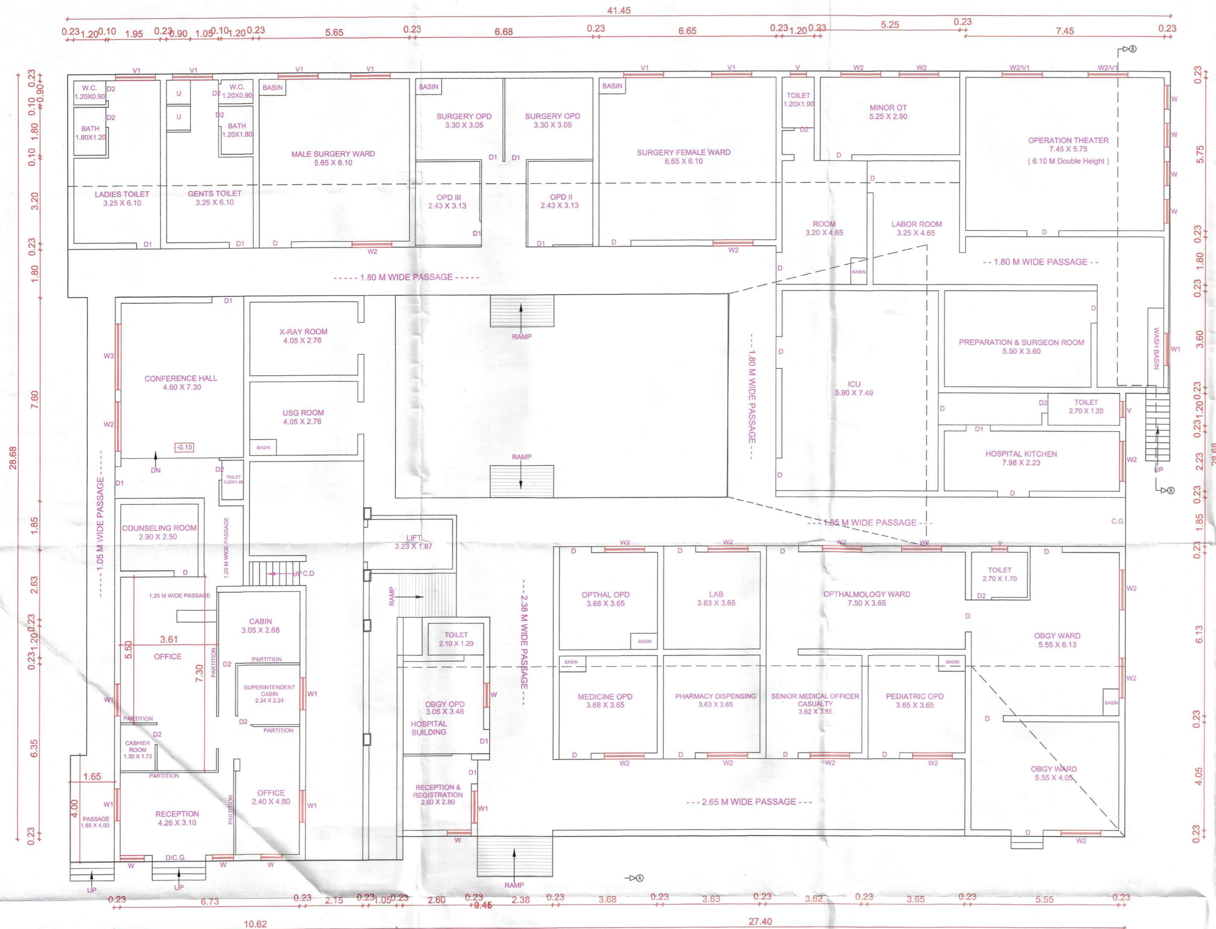
EXISTING. GROUND FLOOR PLAN SCALE - 1:100
